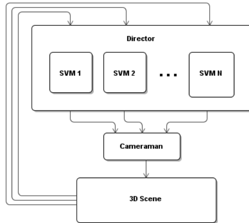
Figure 7. Director Architecture.
